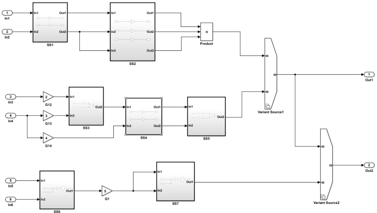
ex_clone_detection
